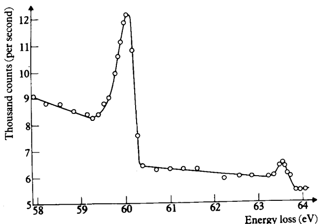
12.9 The energy loss spectrum of 500 eV electrons incident on helium.
